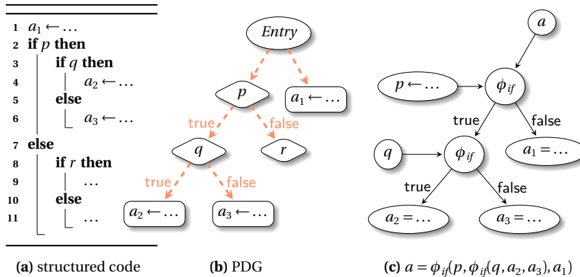
Fig. 12.4 (a) A structured code; (b) the PDG (with region nodes ommited); (c) the DAG representation of the nested gated \phi_{if}
