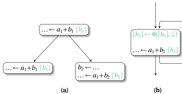
Fig. 9.4 Examples of expression renaming
