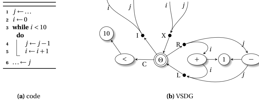
Fig. 12.7 An example showing a for loop. Evaluating X triggers it to evaluate the I value (outputting the value L ). While C evaluates to true, it evaluates the R value (which in this case also uses the \theta -node's L value). When C is false, it returns the final internal value through X . As i is not used after the loop there is no dependency on i at X .
