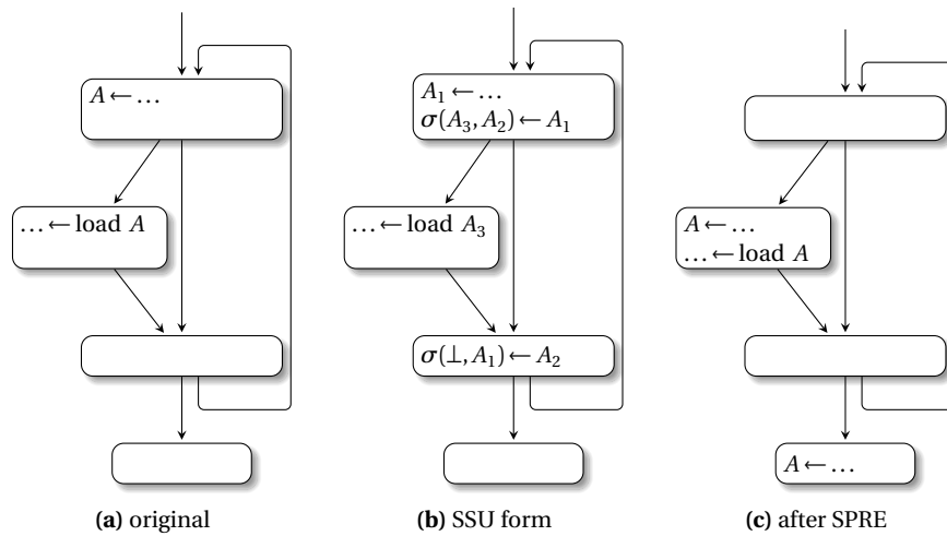
Fig. 9.11 Example of program in SSU form and the result of applying SSUPRE *
