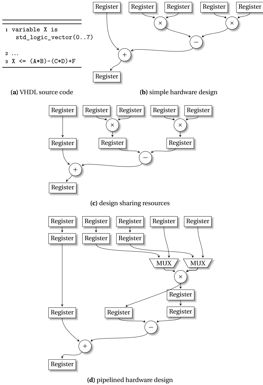
Fig. 18.1 Different variants of mapping a computation to hardware
