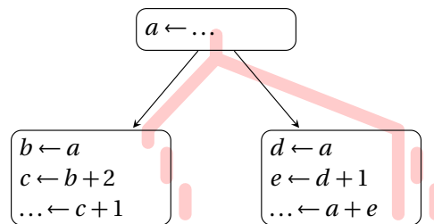
Fig. 17.6 Variables live ranges are sub-trees of the dominator tree*
