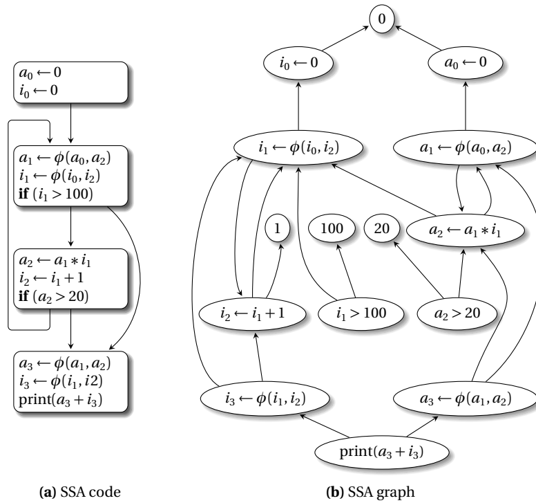
Fig. 12.1 Some SSA code translated into an SSA graph. Note how edges demand the input values for a node.
