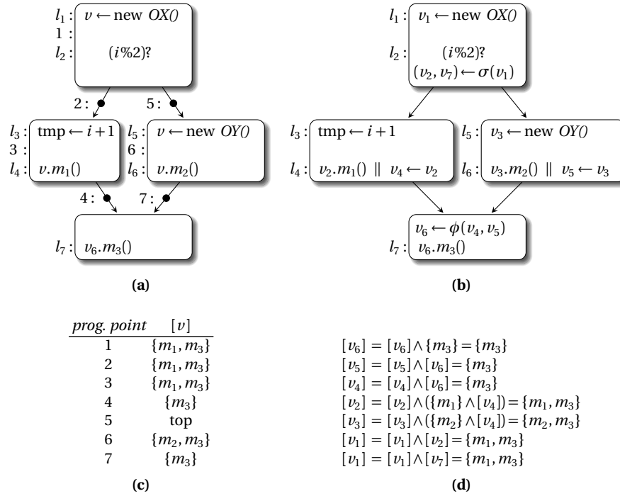
Fig. 11.3 Class inference analysis as an example of backward data-flow analysis that takes information from the uses of variables.
