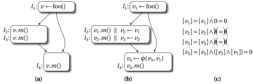
Fig. 11.4 Null pointer analysis as an example of forward data-flow analysis that takes information from the definitions and uses of variables (0 represents the fact that the pointer is possibly null, ! if it cannot be).
