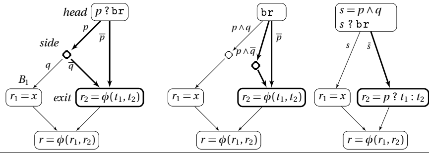
Fig. 16.7 convergent conjunctive merge
