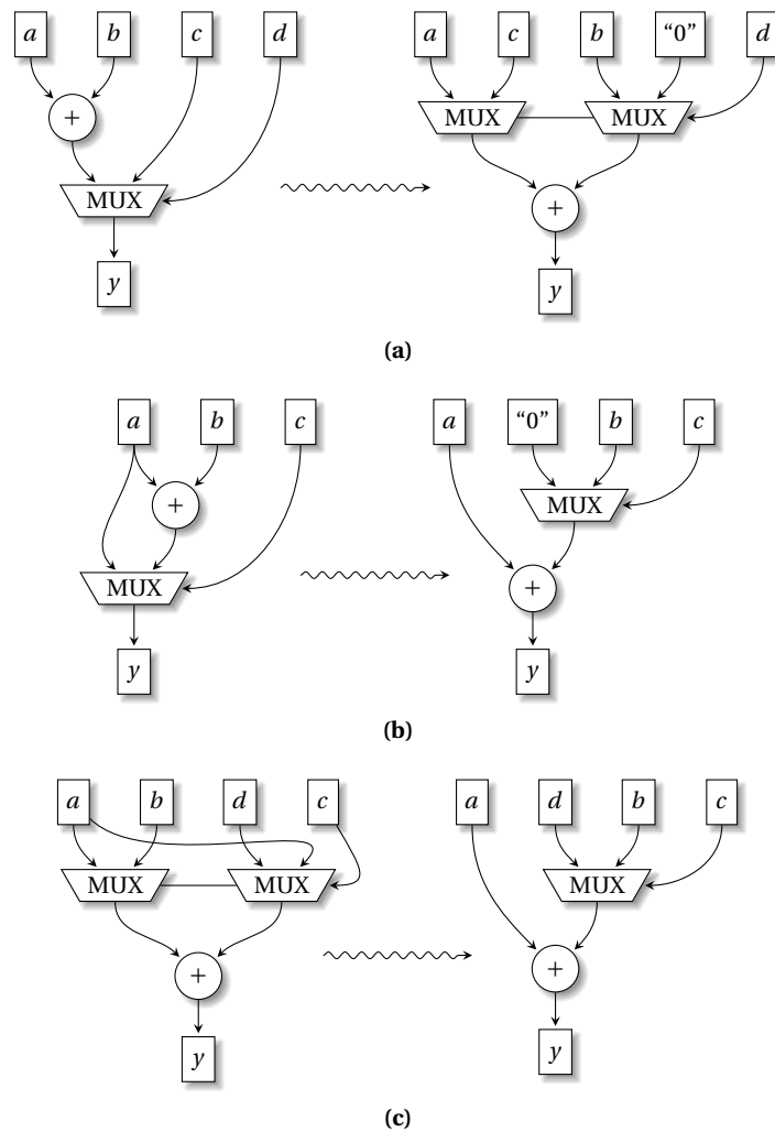
Fig. 18.7 Multiplexer-Operator transformations: juxtaposition of a multiplexer and an adder (a,b); reducing the number of multiplexers placed on the input of an adder (c)
