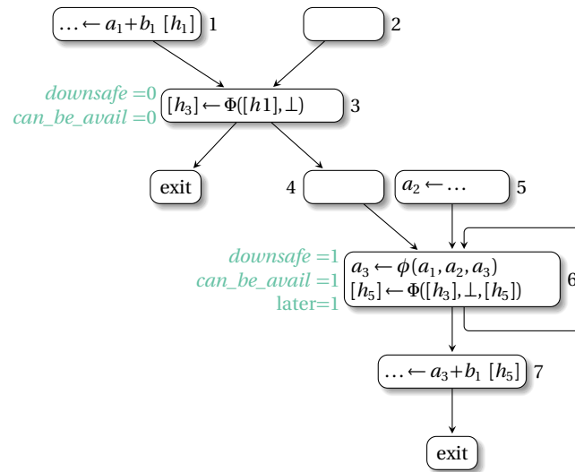
Fig. 9.5 Example to show the need of the later attribute
