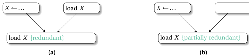
Fig. 9.9 Redundant loads after stores
