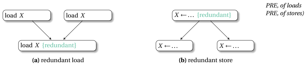
Fig. 9.8 Duality between load and store redundancies
