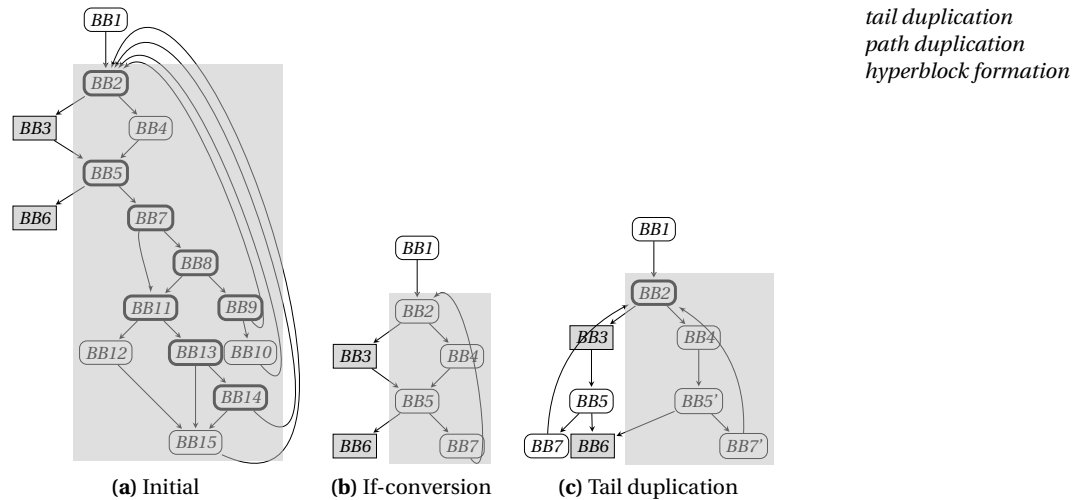
Fig. 16.11 If-conversion of wc (word count program). Basic blocks in the gray region cannot be if-converted. Tail duplication can be used to exclude BB3 from the to-be-if-converted region.
