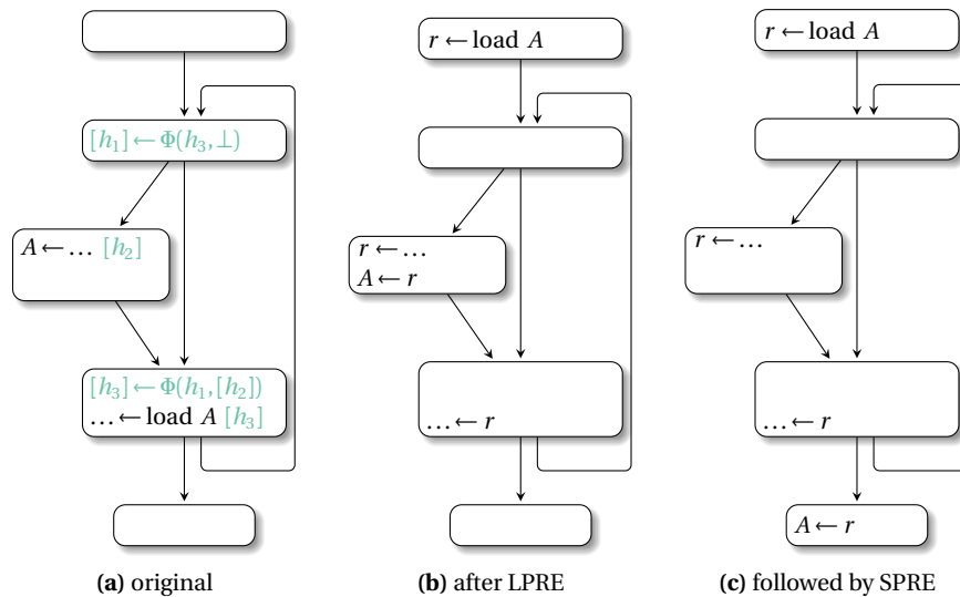
Fig. 9.10 Register promotion via load PRE followed by store PRE
