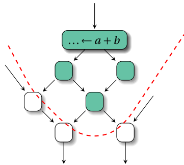
Fig. 9.2 Dominance frontiers (dashed) are boundaries between fully (highlighted basic blocks) and partially redundant regions (normal basic blocks).
