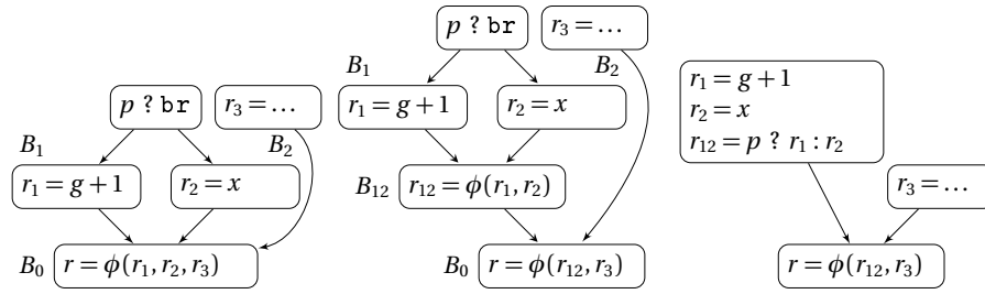
Fig. 16.5 \phi reduction
