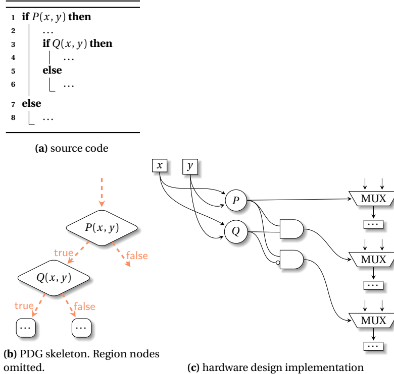
Fig. 18.6 Use of the predicates in region nodes of the PDG for mapping into the multiplexers associated with each \phi -function
