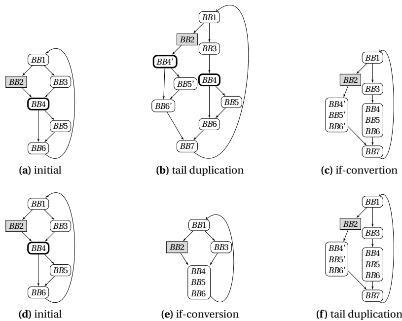
Fig. 16.12 Absence of phasing issue for tail duplication
