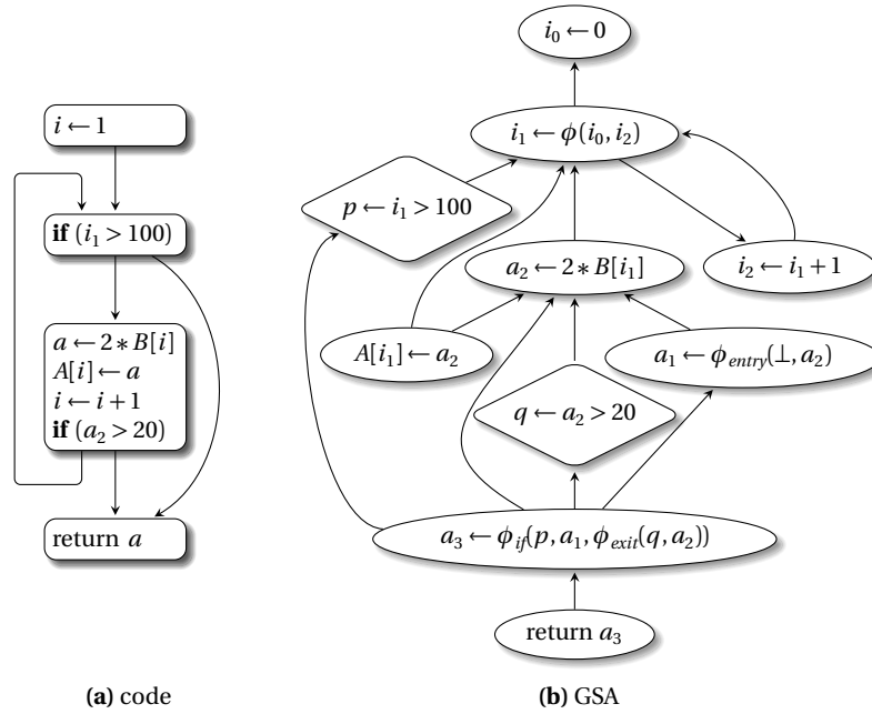
Fig. 12.3 A graph representation of our sample code in (demand-based) GSA form.
