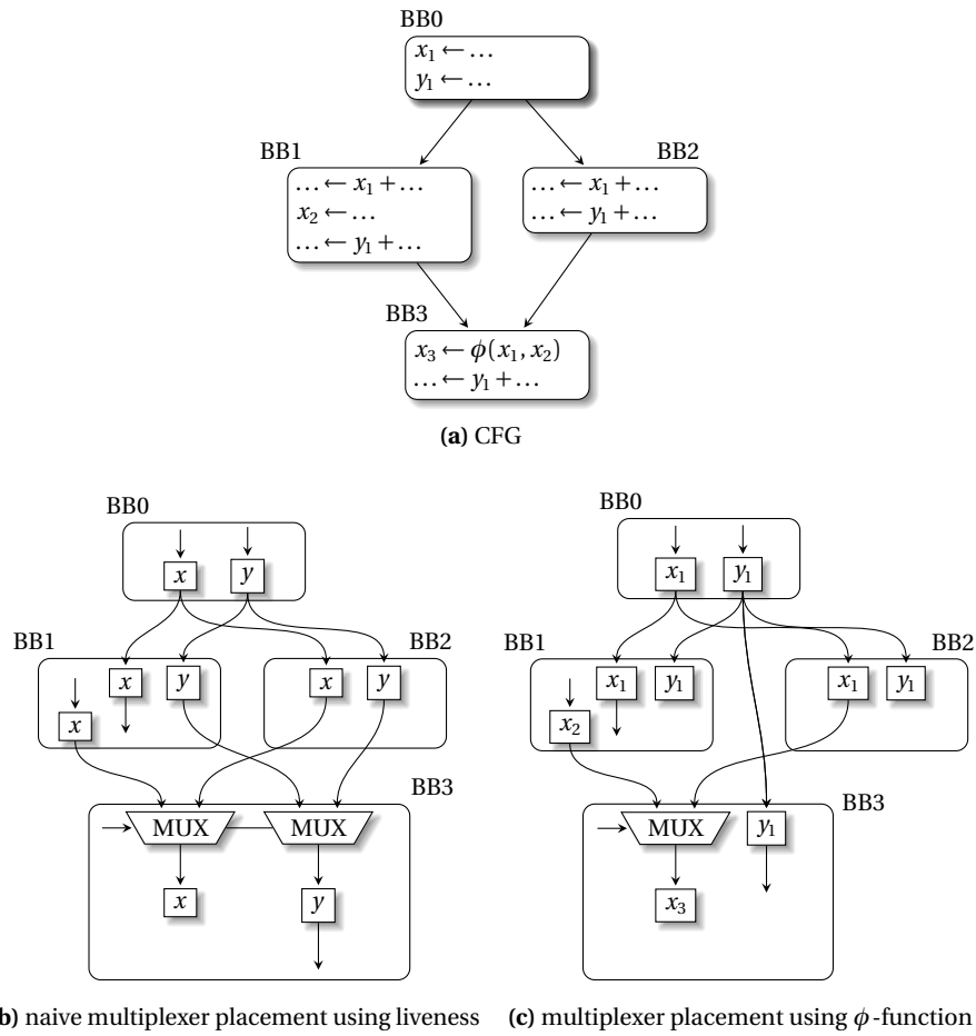
Fig. 18.4 Mapping of variable values across hardware circuit using spatial mapping
