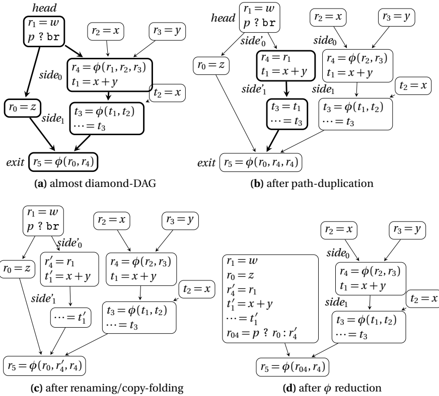
Fig. 16.6 Path duplication
