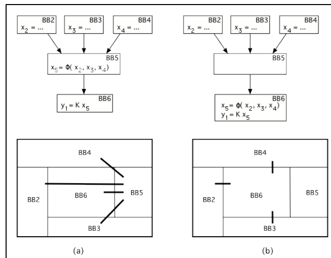
Fig. 18.8 Example of the impact of \phi -function movement in reducing hardware wire length
