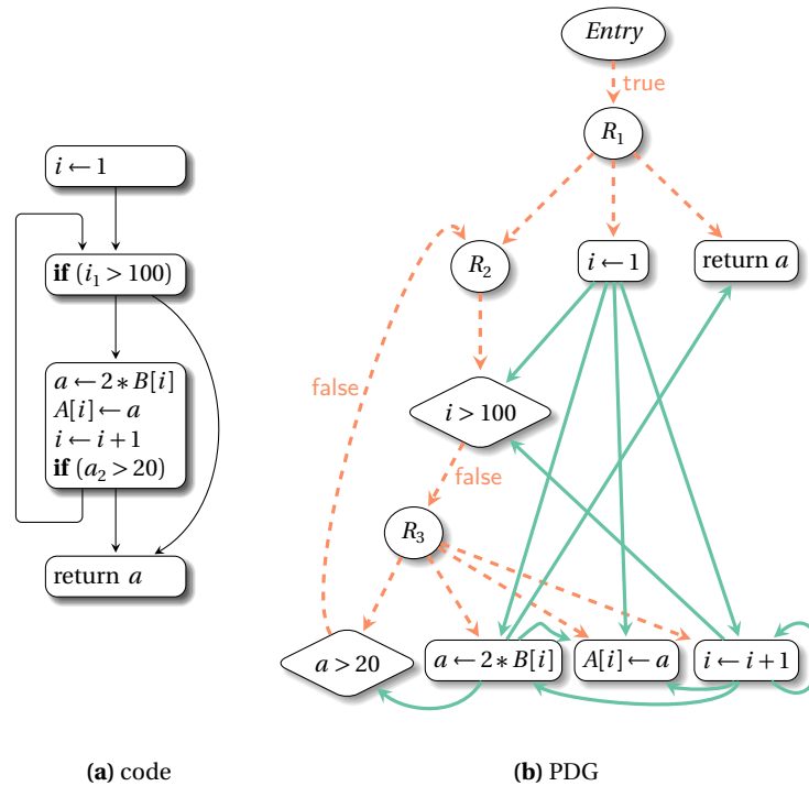
Fig. 12.2 Example code translated into a PDG. Dashed/full edges respectively represent control/data dependencies.
