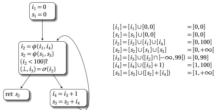
Fig. 11.2 Live-range splitting on Figure 11.1 and a solution to this instance of the range analysis problem.
