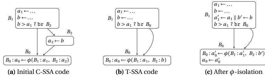
Fig. 17.3 Copy-folding followed by empty block elimination can lead to SSA code for which destruction is not possible through simple copy insertion
