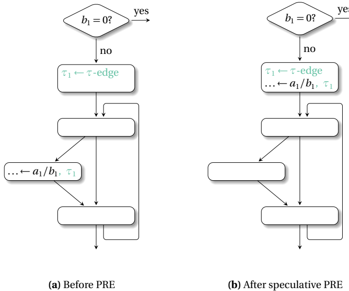
Fig. 9.7 Speculative and fault-safe loop-invariant code motion
