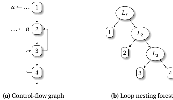
Fig. 7.2 Bad case for iterative data-flow analysis.
