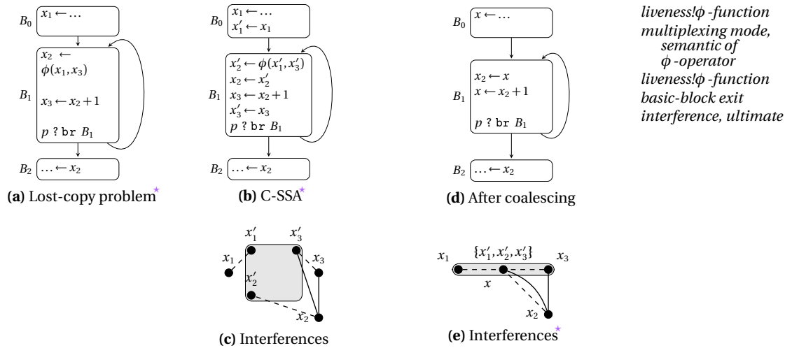
Fig. 17.5 SSA destruction for the lost-copy problem.
