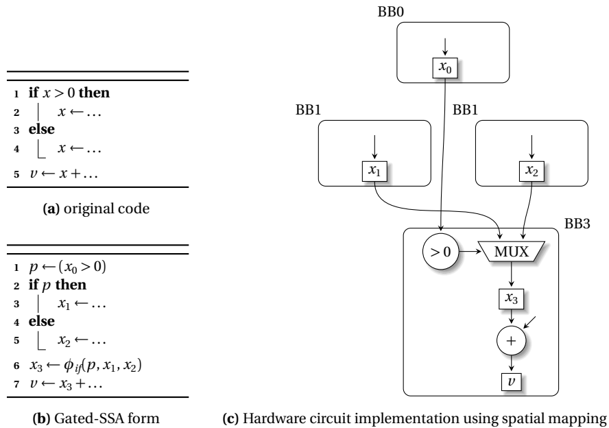
Fig. 18.5 Hardware generation example using Gated-SSA form
