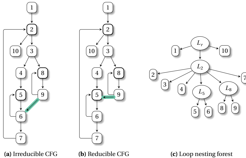
Fig. 7.3 A reducible CFG derived from an irreducible CFG, using the loop nesting forest. The transformation redirects edges arriving inside a loop to the loop header (here 9 \rightarrow 6 into 9 \rightarrow 5 ).
