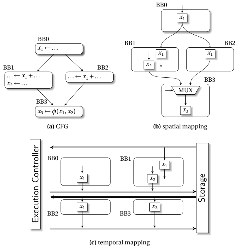
Fig. 18.3 Combination of hardware circuits for multiple basic blocks
