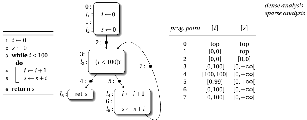
Fig. 11.1 An example of a dense data-flow analysis that finds the range of possible values associated with each variable at each program point.
