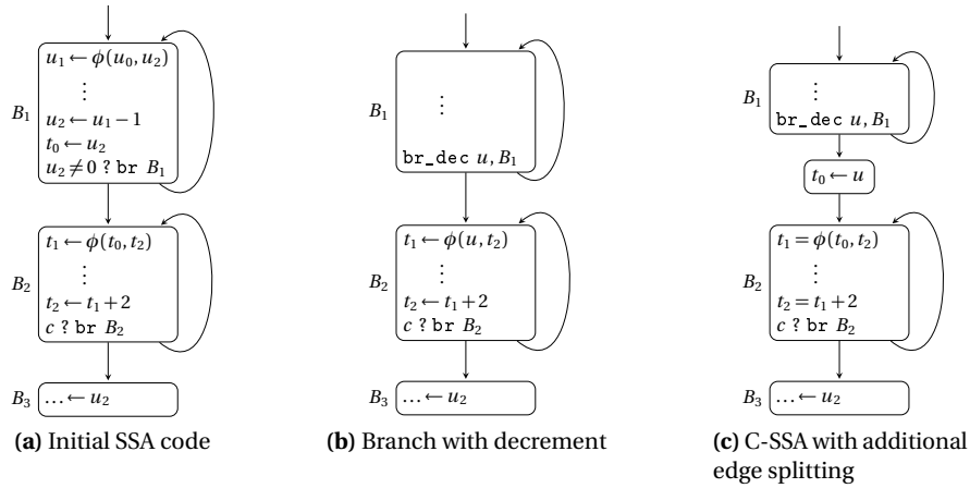
Fig. 17.2 Copy insertion may not be sufficient. \text{br\_dec } u, B_1 decrements u , then branches to B_1 if u \neq 0 .
