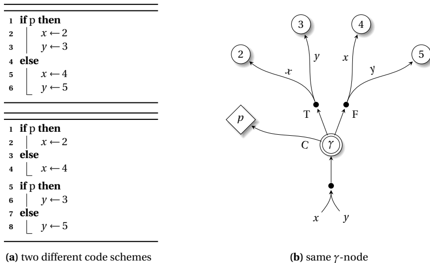
Fig. 12.6 Two different code schemes map to the same \gamma -node structure.
