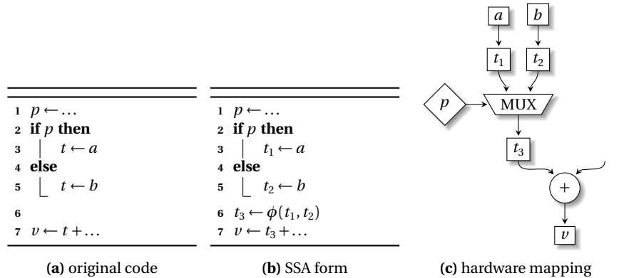
Fig. 18.2 Basic hardware mapping using SSA representation
