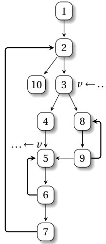
Fig. 7.1 An example of a reducible CFG. Forward CFG is represented using full edges; back-edges are thickened. Backward pass on forward CFG sets v as live-in of node 5, but not of node 2. Forward pass on loop nesting forest then sets v as live at node 6 but not at node 7.
