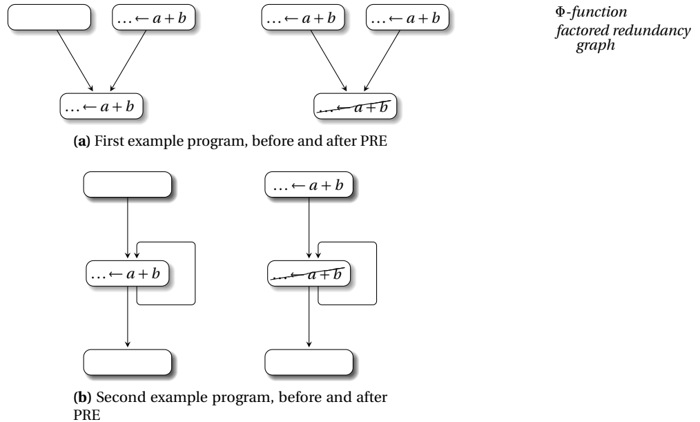
Fig. 9.1 Two basic examples of partial redundancy elimination.
