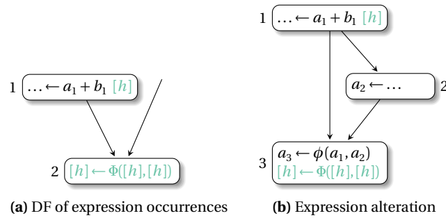
Fig. 9.3 Examples of \Phi insertion
