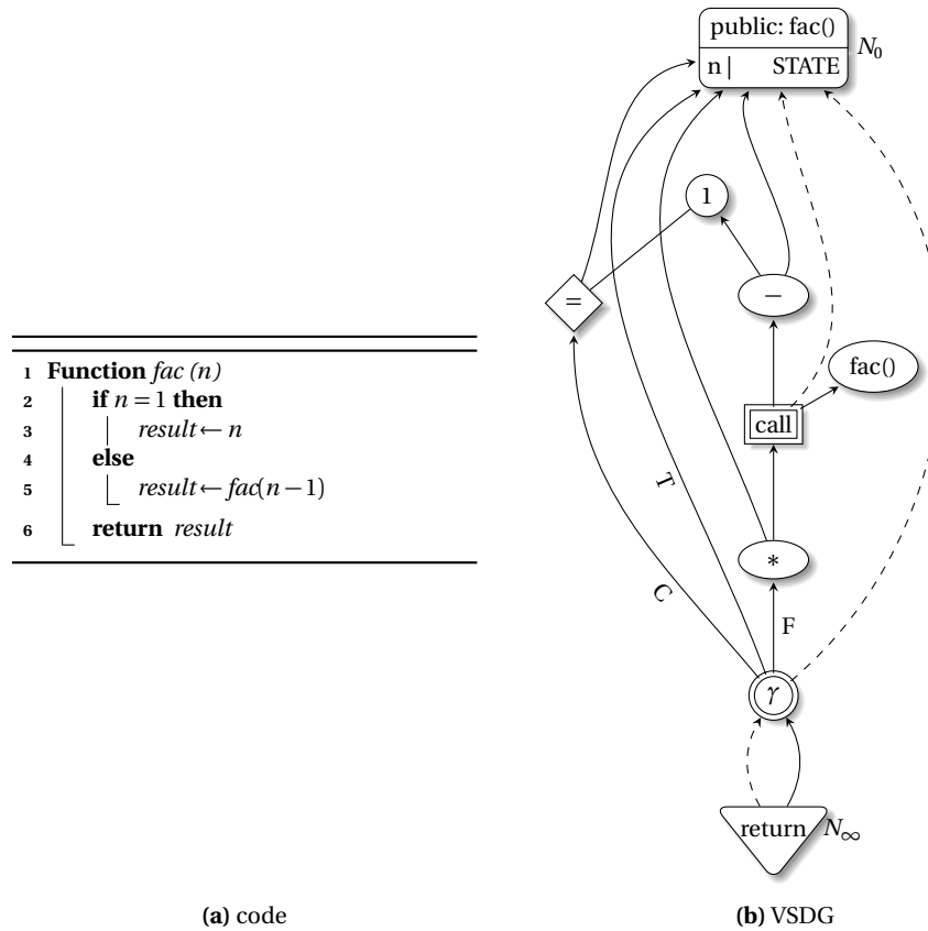
Fig. 12.5 A recursive factorial function, whose VSDG illustrates the key graph components—value dependency edges (solid lines), state dependency edges (dashed lines), a call node, a const node, a \gamma -node, a conditional node, and the function entry and exit nodes.
