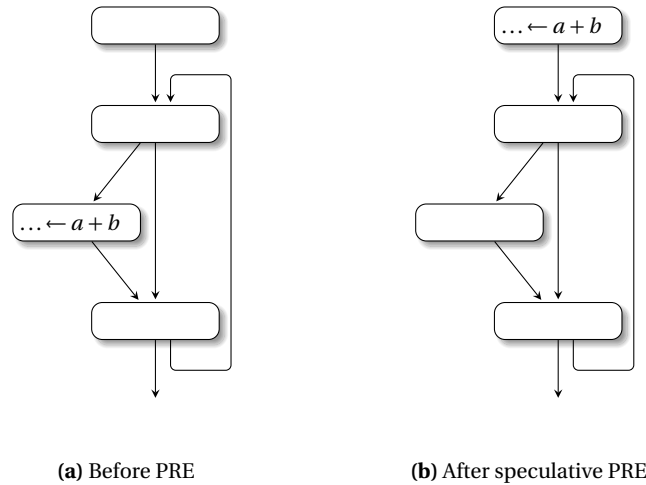
Fig. 9.6 Speculative loop-invariant code motion
