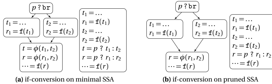
Fig. 16.8 SSA predicate minimality
