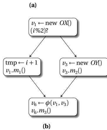
Fig. 11.10 (a) implementing \sigma -functions via single arity \phi -functions; (b) getting rid of copies and \sigma -functions.
