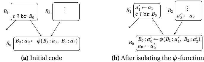
Fig. 17.1 Isolation of a \phi -node*
